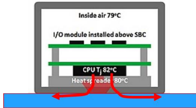
Figure 2: Conduction cooling for rugged electronics enclosure
